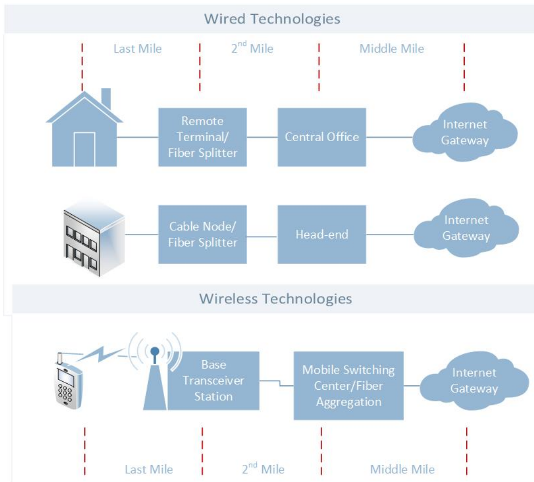
Figure 7. Wired and Wireless Connections
