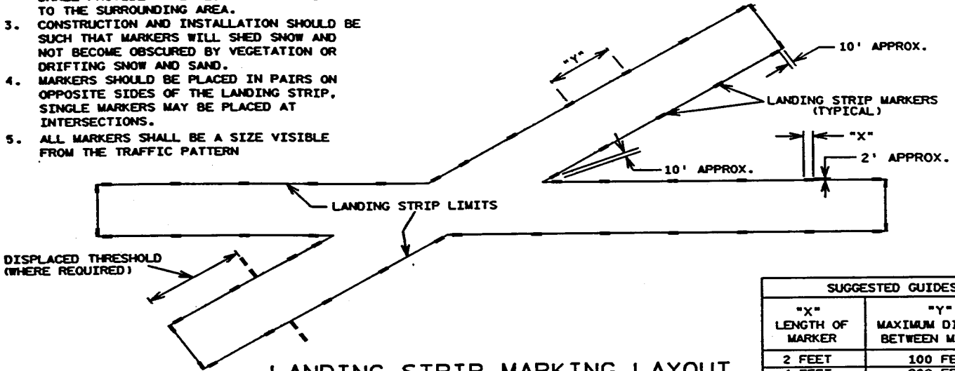
LANDING STRIP MARKING LAYOUT
