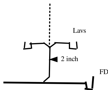
Common vents serving as a wet vent
