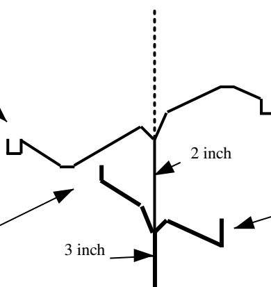
Common vents serving as a wet vent
