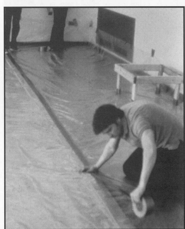
Figure 8.3a Prepare the Worksite With Plastic Sheetting (interior).
