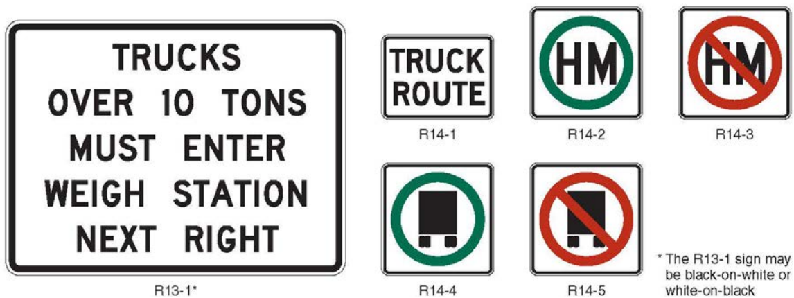
Figure 2B-30. Truck Signs
