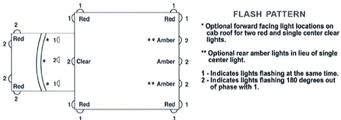
Figure 1 – Emergency Lighting
